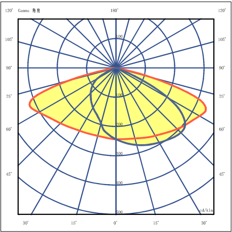
T3M light distribution curve
