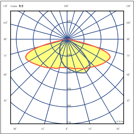
T2S light distribution curve
