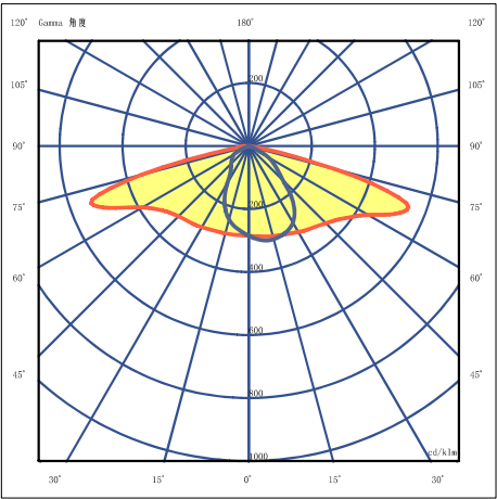
T2M light distribution curve
